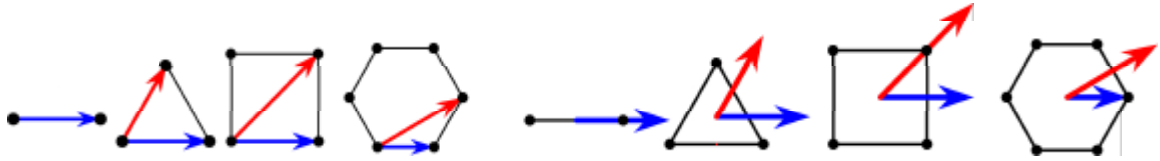
Fig. 1 Left: Regular polygons n = 1, 2, 3, 4, 6 with vector generators a, b . Right: a, b attached to polygon centers.
