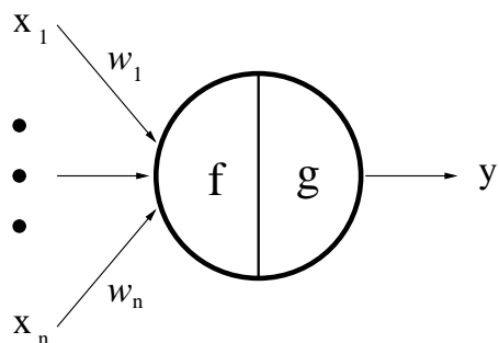
Figure 3.1: Model of a generic neuron.
